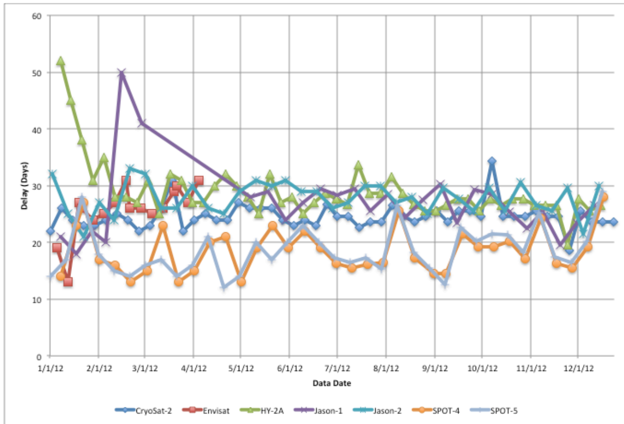
Figure 2. Delay in delivery of DORIS data to the CDDIS (all satellites, 01-12/2012)
